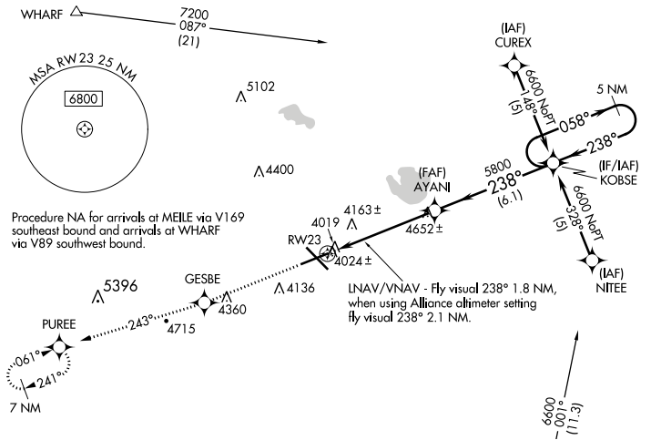
RNAV Approach
